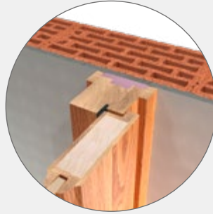
RAHMENSTOCK Türblatt massiv
