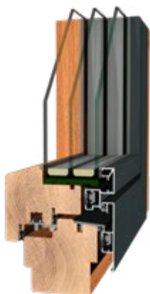
QG HOLZ-ALU FLAT Uf-Wert = 1,03 W/m 2 K
